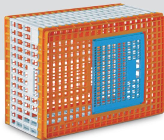
Mini Piedmont Coop Dimensions: 30 5/16 x 22 7/16 x 11 in and 30 5/16 x 22 7/16 x 13 in
